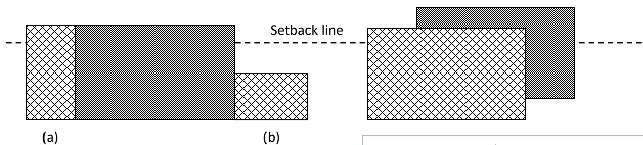
Figure 2: a) NC structure addition that does not encroach further into the setback than existing structure, OR b) NC structure addition that does not extend into the setback at all. (Sec. 3.8.B.1)
