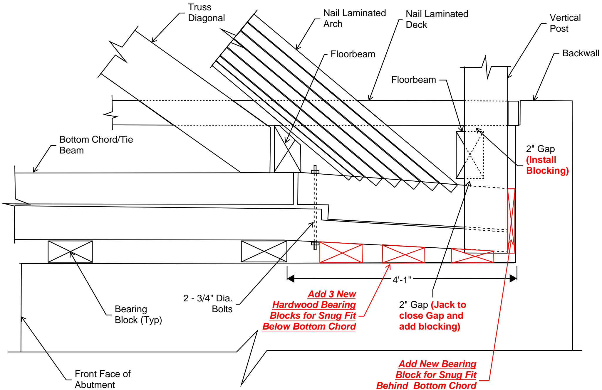
SOUTHWEST TRUSS BEARING DETAIL LOOKING EAST NTS
